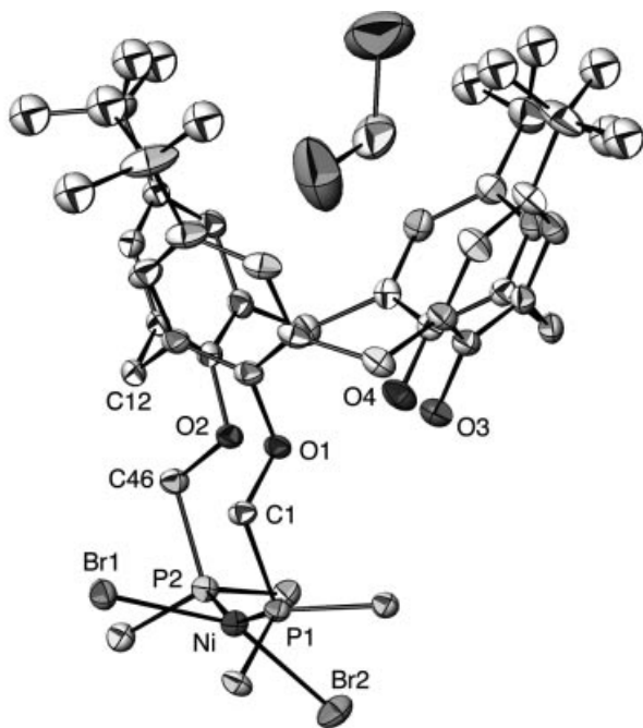
Figure 2. Molecular structure of the turquoise complex [\text{NiBr}_2\cdot\mathbf{1}]\cdot 2\text{CH}_2\text{Cl}_2 ( 3 · 2\text{CH}_2\text{Cl}_2 ); for clarity, only the \text{C}_{\text{ipso}} atoms of the P-phenyl rings are shown; the t Bu groups are not shown in full
