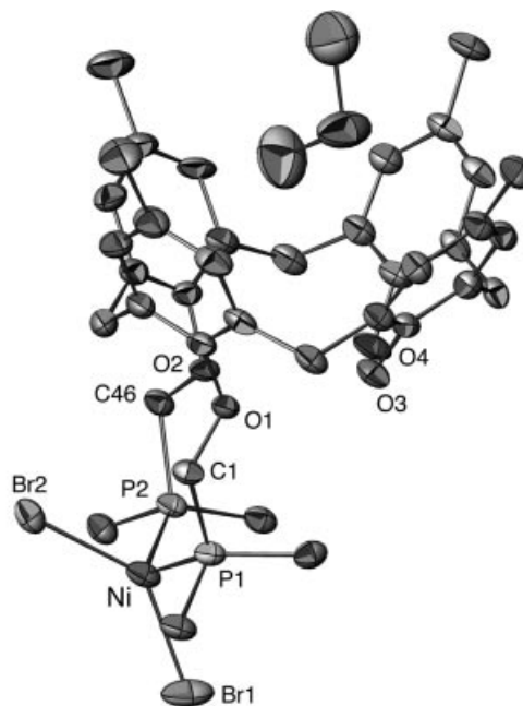
Figure 3. Molecular structure of the red brown complex [\text{NiBr}_2\cdot\mathbf{1}]\cdot 1.75\text{CH}_2\text{Cl}_2 ( 4 · 1.75\text{CH}_2\text{Cl}_2 ); for clarity, only the \text{C}_{\text{ipso}} atoms of the P-phenyl rings are shown; the t Bu groups are not shown in full
