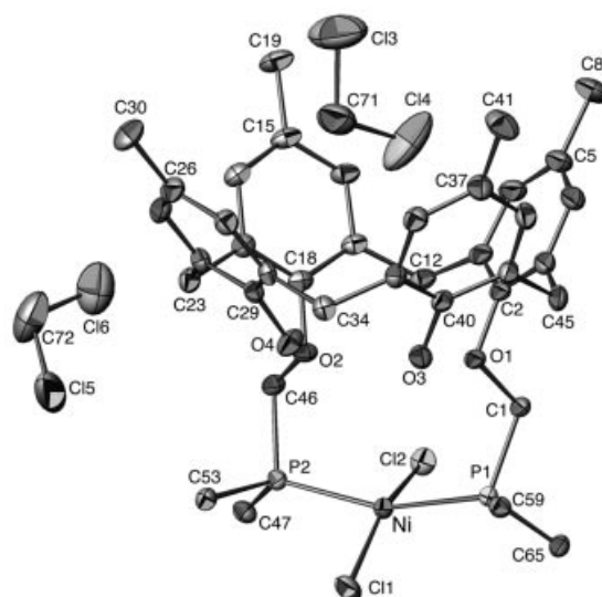
Figure 1. Molecular structure of the blue complex [\text{NiCl}_2 \cdot \mathbf{1}] \cdot 2\text{CH}_2\text{Cl}_2 ( \mathbf{2} \cdot 2\text{CH}_2\text{Cl}_2 ); only the \text{C}_{\text{ipso}} atoms of the P-phenyl rings are shown; the t Bu groups are not shown in full
